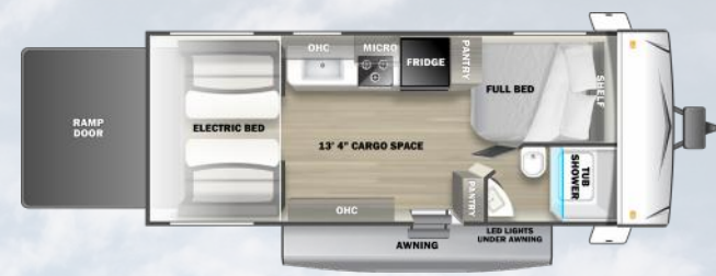
CB1913 (13' 4" CARGO)
